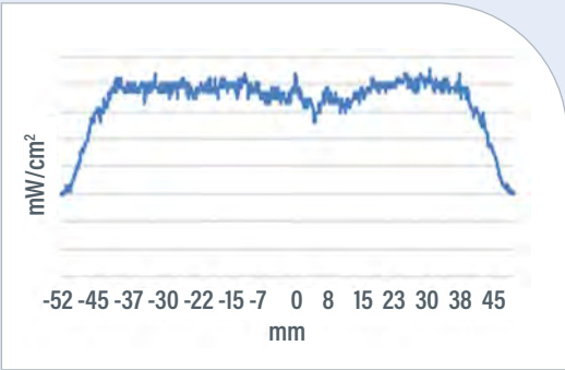
Intensity Response at 25-mm Working Distance 1-mm Mounting Gap
