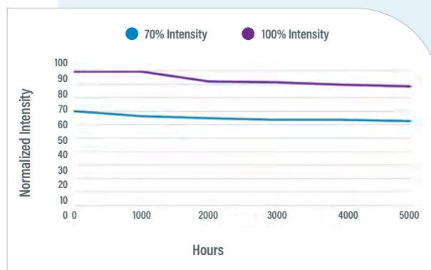
Figure 9. LED Degradation Testing - RediCure
