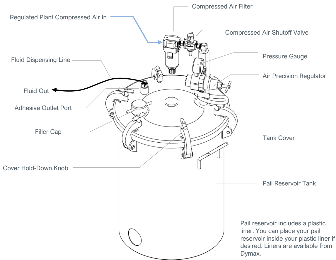
Figure 6. Pail Reservoir Tank Components
