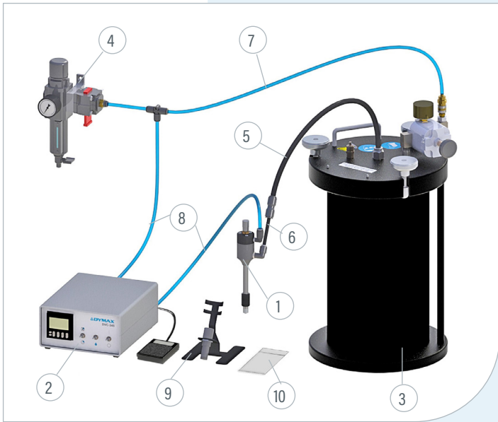
Representative Model 400 Dispensing System (T17707 with Bottle Drop-in Reservoir Shown Below)
