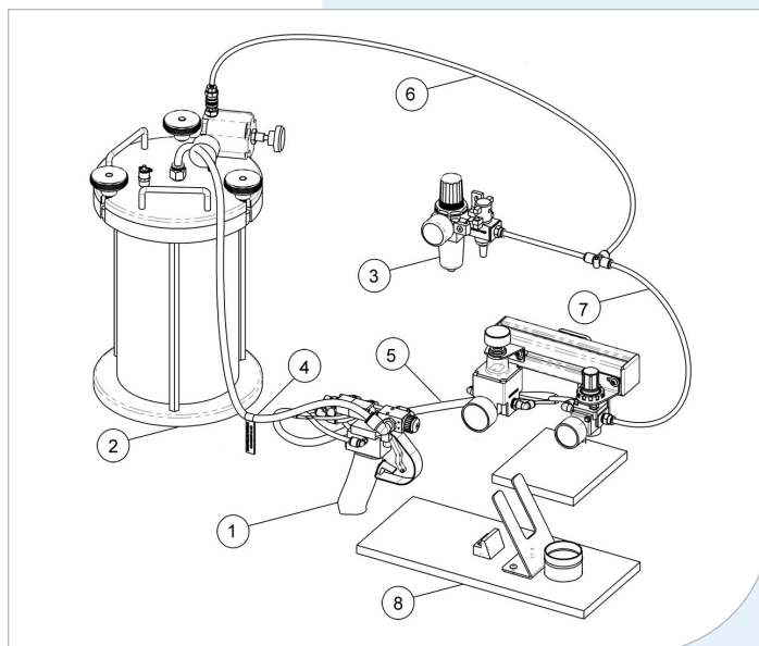
Representative SG150-RS Spray Dispensing System (T18455 with Large Bottle Reservoir Shown Below)
